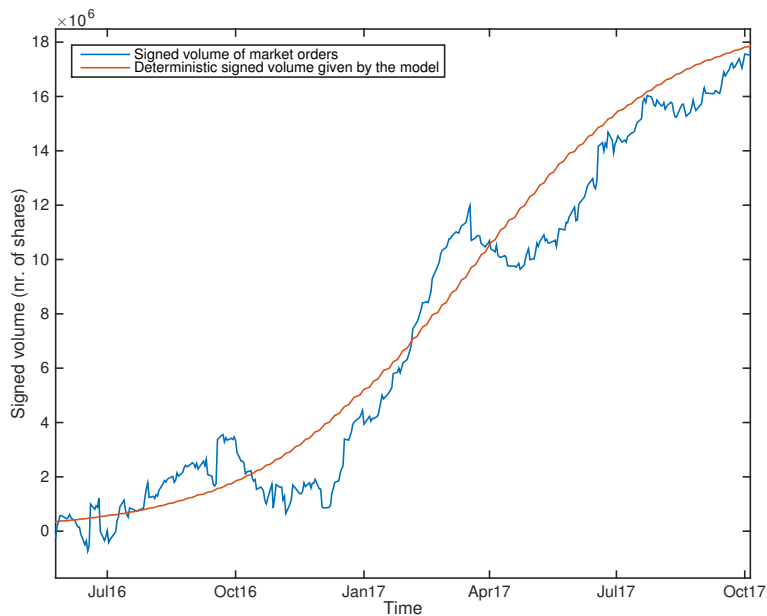
Figure 4.18: Realized signed volume of market orders and deterministic signed volume given by equation (4.11), Amazon.com Inc, June 2016 - October 2017.
