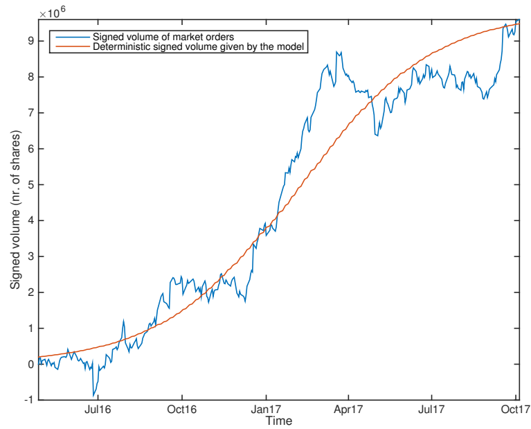
Figure 4.17: Realized signed volume of market orders and deterministic signed volume given by equation (4.11), Alphabet Inc, June 2016 - October 2017.
