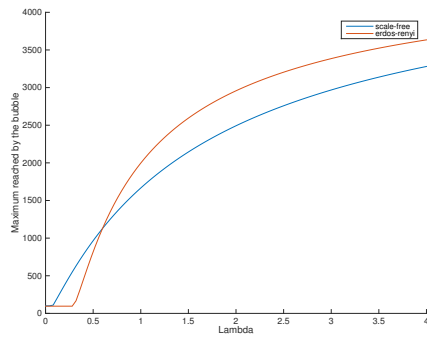
Figure 4.2: Maximum value of the bubble as a function of \lambda with \delta = 1 , k = 0.4 .
