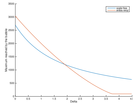
Figure 4.3: Maximum value of the bubble as a function of \delta with \lambda = 1 , k = 0.4 .
