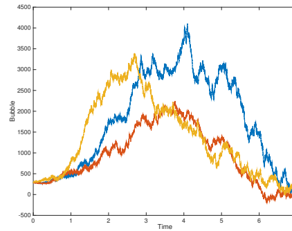
Figure 4.14: Example of trajectories for a bubble in an Erdős-Rényi network.
