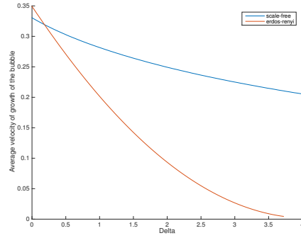
Figure 4.6: Average velocity of growth as a function of \lambda , with \delta = 1 , k = 0.4 . Figure 4.7: Average velocity of growth as a function of \delta , with \lambda = 1 , k = 0.4 .
