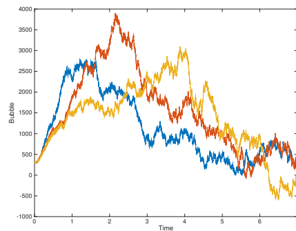
Figure 4.12: Corresponding trajectories of the bubble in a scale-free network with mean degree z = 3.2 .
