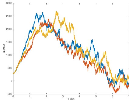
Figure 4.13: Example of trajectories for a bubble in a scale-free network.
