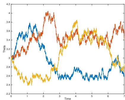
Figure 4.11: Example of trajectories of \theta with \mu^\theta = 0 , \sigma^\theta = 0.2 .
