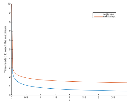
Figure 4.9: Time to the maximum, \lambda = 1 , \delta = 1 , \theta = 1
