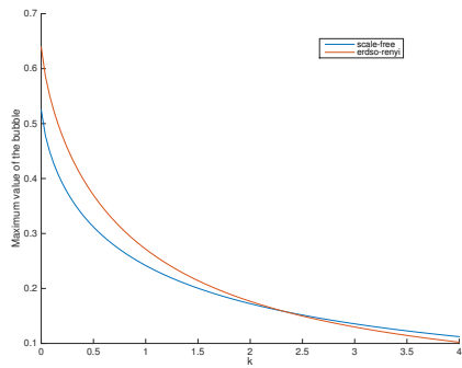
Figure 4.8: Maximum value of the bubble, \lambda = 1 , \delta = 1 , \theta = 1 .
